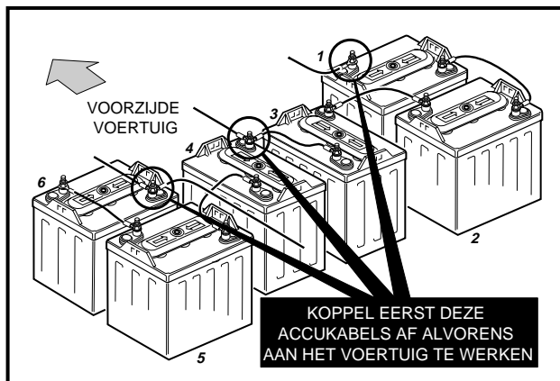
Figuur 1 V-Glide 36-Volt Vehicle
